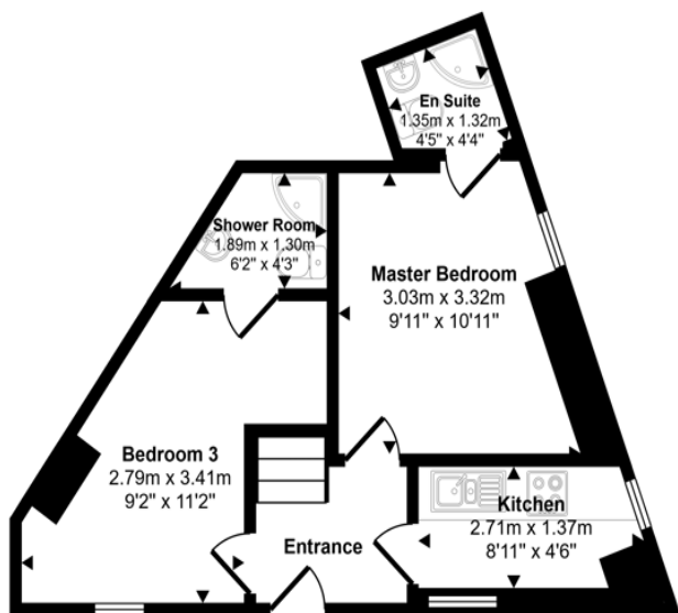
Ground Floor Approx 32 sq m / 341 sq ft
