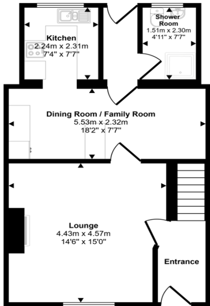
Ground Floor Approx 53 sq m / 572 sq ft
